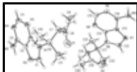
Fig. 1. View of the title compound without the hydrogen atom-labeling scheme. Displacement ellipsoids are drawn at the 30% probability level.
