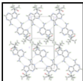
Fig. 2. A view of the molecular packing along a axis.
